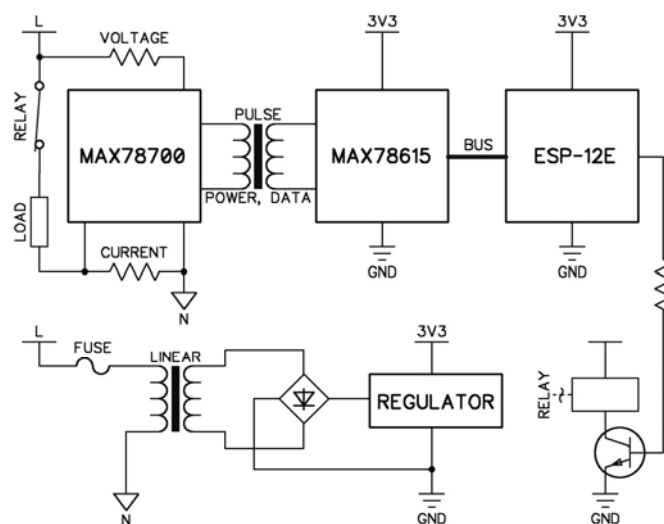
Fig. 6 The proposed block diagram of a client node
