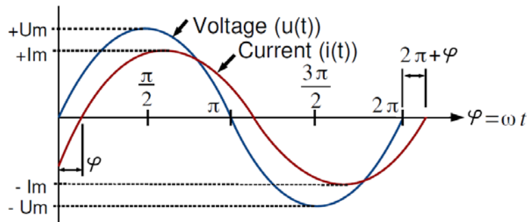
Fig. 2 The phase difference between voltage (blue) and current (red)
